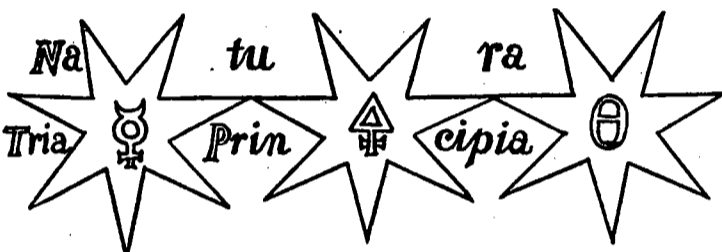
the Root of all Metals.
